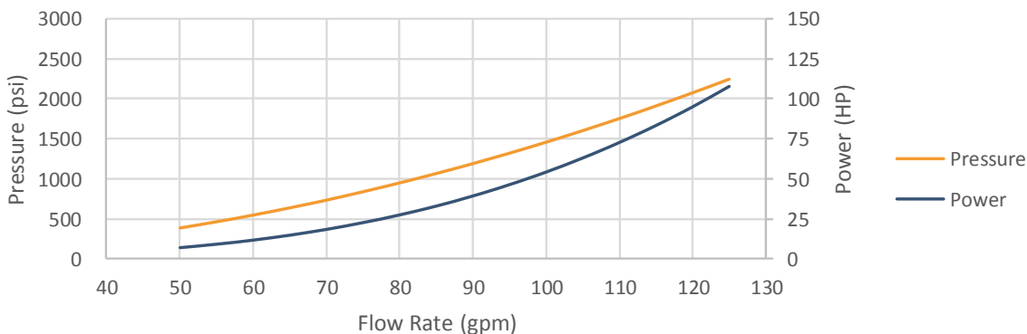
2-7/8"-3D-90 Turbodrill Nominal Outputs with 8.33ppg WBM
