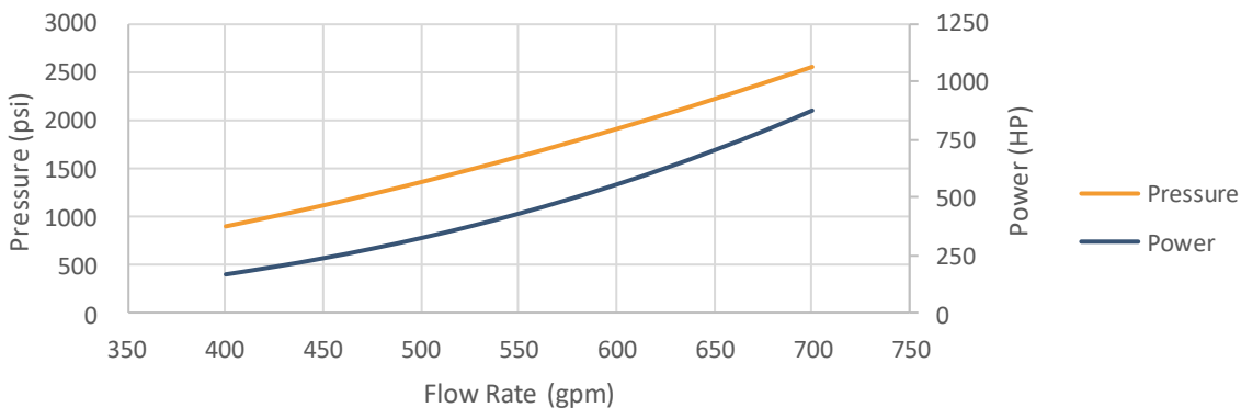
6-3/4"-3D-106 Turbodrill Nominal Outputs with 10ppg WBM
