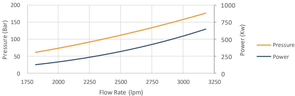
172-3D-106 Turbodrill Nominal Outputs with 1,2 SG WBM
